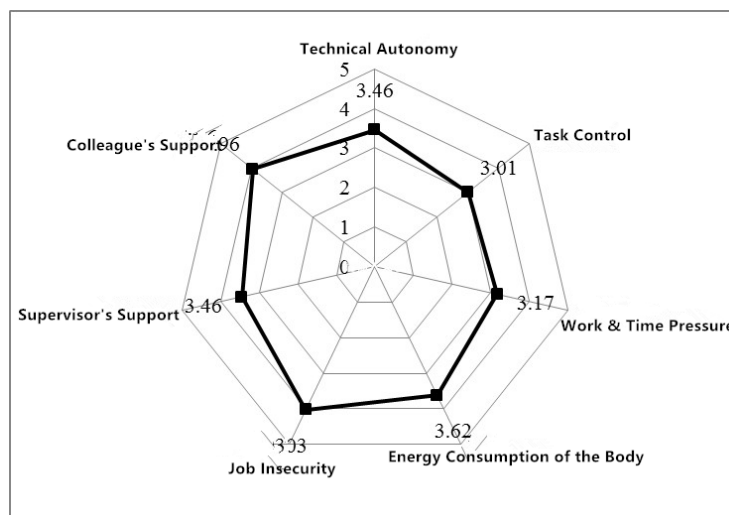
Fig. 1. Radar chart of the average value of the multi-dimensions of the quality of work and life of tourism consultants
